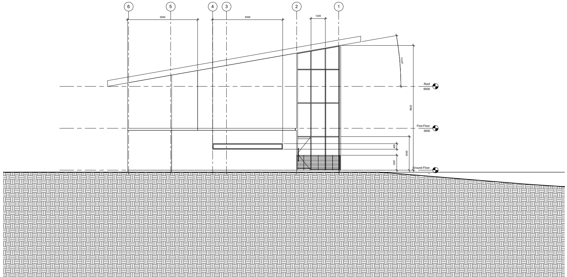
1 EAST ELEVATION 1 : 50
