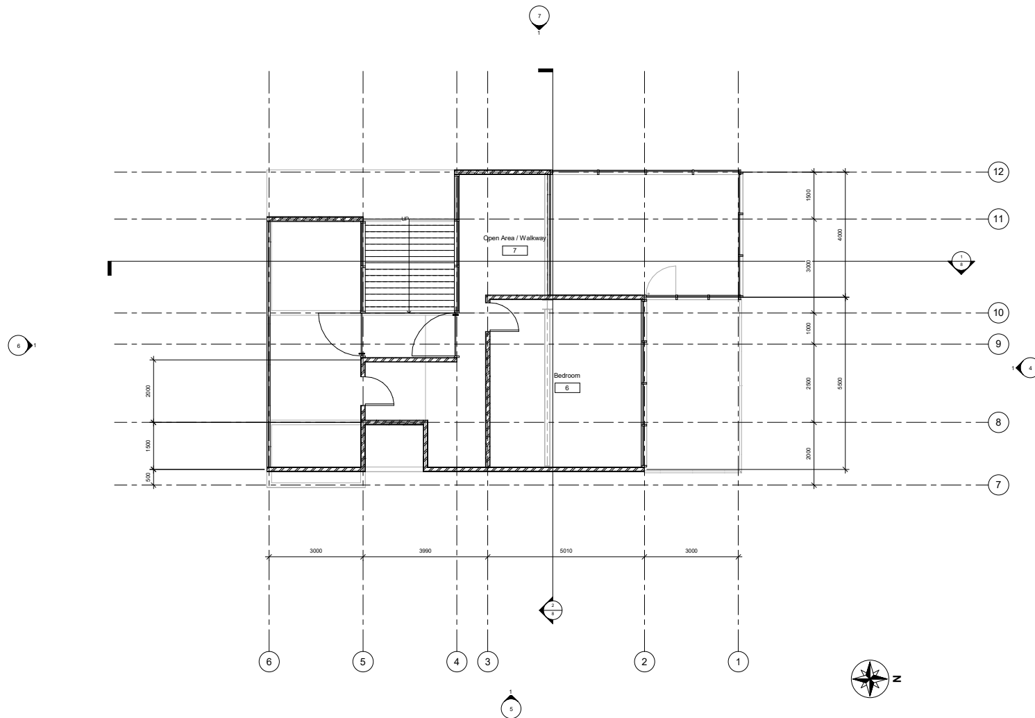
1 First Floor 1 : 50
